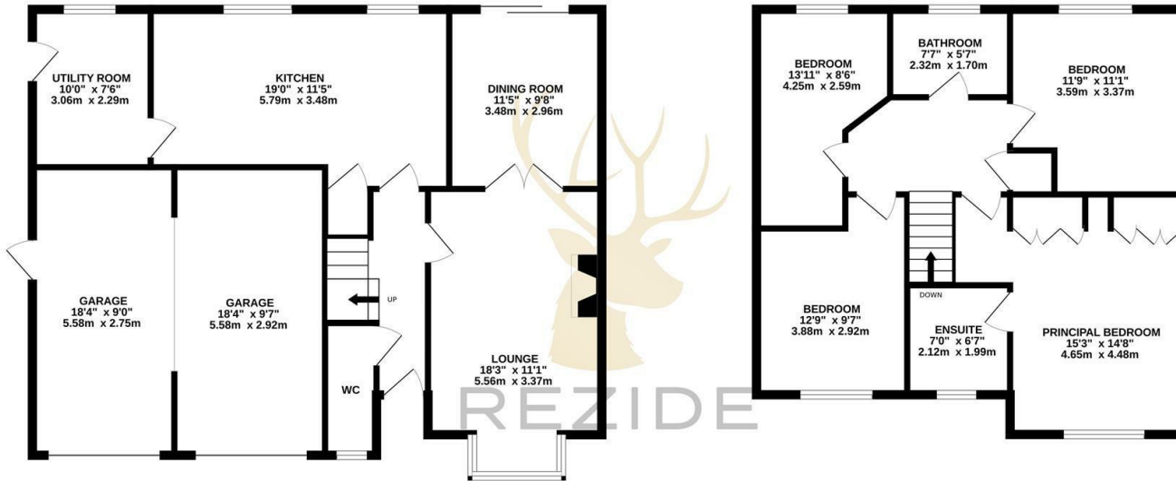
GROUND FLOOR 1007 sq.ft. (93.5 sq.m.) approx.
